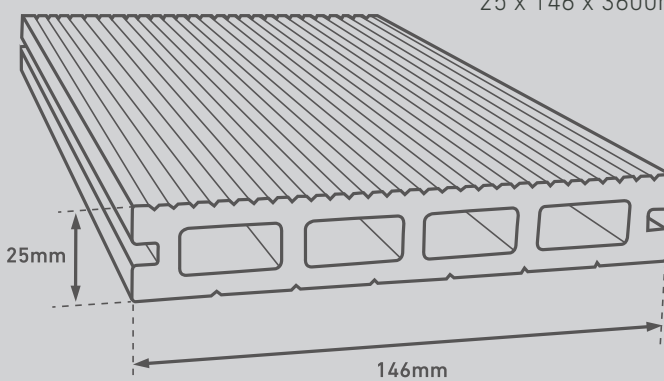
Board Dimension 25 x 146 x 3600mm
